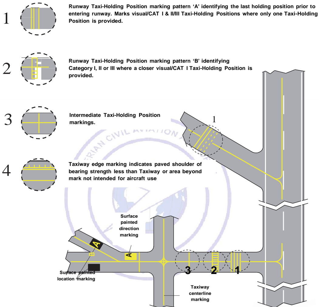
Figure 2.2 Paved Taxiway Markings (not to scale)
