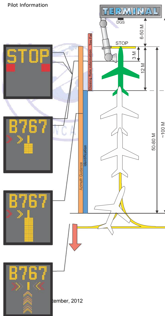
Figure 4.4 Safedock Guidance System
