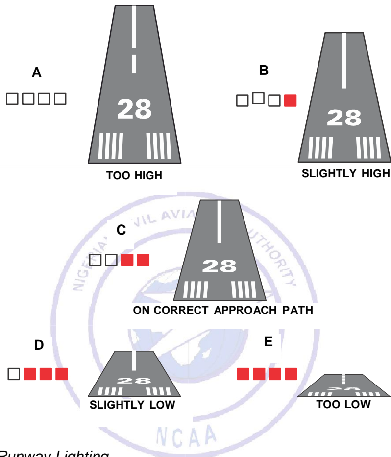
Figure 1.4 A Typical PAPI System
