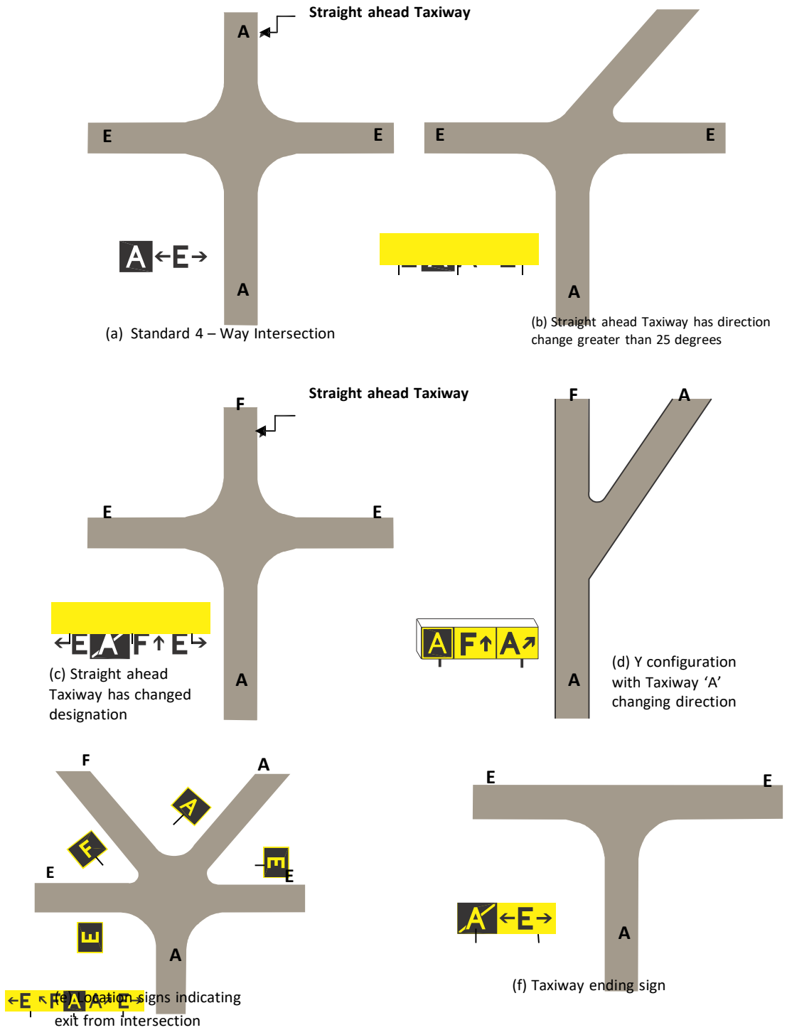
Figure 3.4 Examples of Taxi Guidance Signs at Taxiway Intersections (not to scale)
