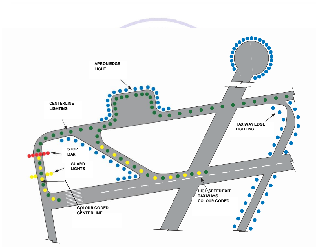
Figure 1.7 Taxiway Lighting
