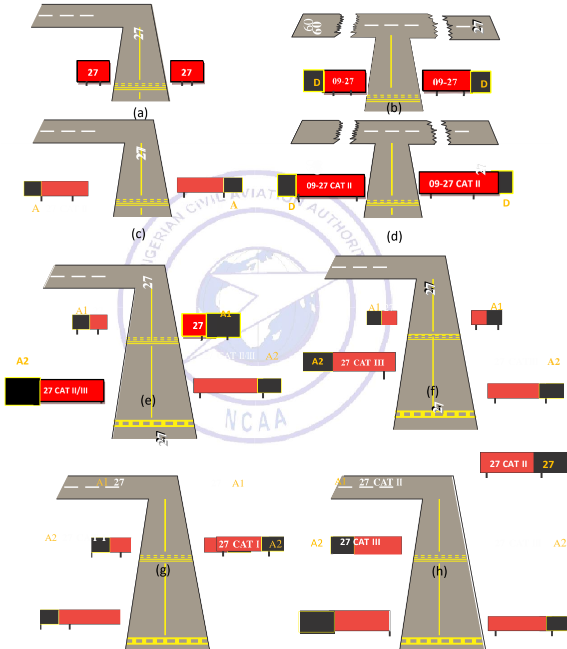
Figure 3.2: Typical Runway Holding Position Signs and Associated Taxiway Markings.
