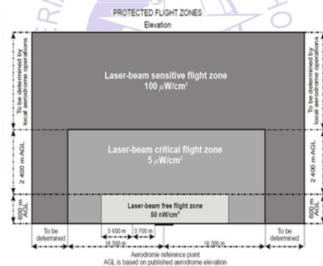
Figure 1-3 Protected flight zones with indication of maximum
