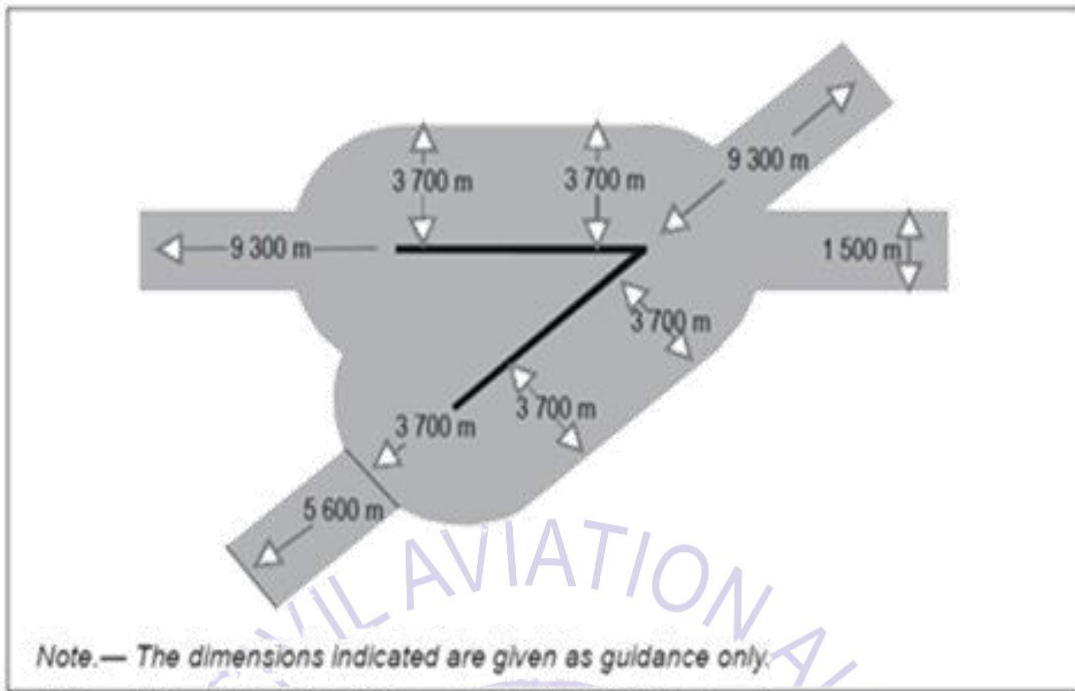
Figure 1-2 Multiple runway laser-beam free flight zones
