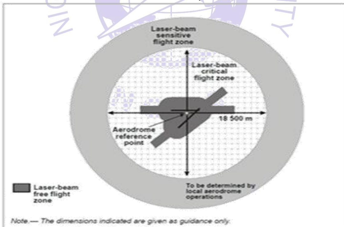
Figure 1-1: Protected flight zones
